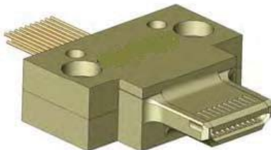
LVDS-Plug, 2-channel (without mounting shoe, Part No. 18198)
